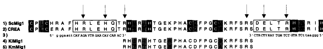
Fig. 1. Amino acid sequences of the zinc finger regions from S. cerevisiae Mig1 (line 1) and A. nidulans CREA protein (line 2). The cysteine and histidine residues of the C 2 H 2 motifs are highlighted in black boxes and the divergent residues are stippled. Residues thought to be in contact with the GC-rich MIG1-binding site are marked by arrows. The 6 identical residues used to design the degenerate primers (line 3) are boxed (M = A or C; R = A or G; Y = C or T). Unpaired nucleotides providing Eco RI sites are shown in lower case. Lines 4 and 5 show the amino acid sequences of the PCR fragments from K. lactis and K. marxianus , respectively.
